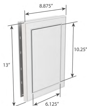
Large Mounting Block
