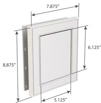
Standard Mounting Block
